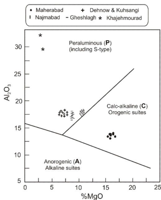
Fig 7. \text{Al}_2\text{O}_3 -MgO biotite discrimination diagram, Abdel-Rahman [5].
