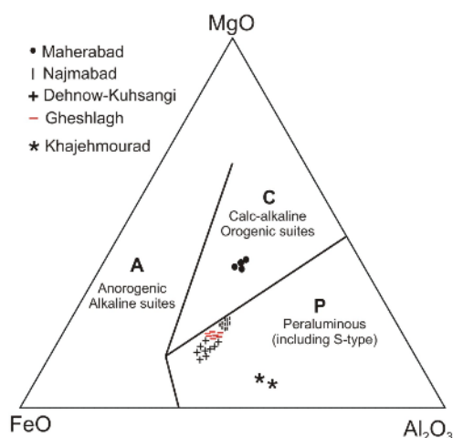
Fig 8. Distribution of micas on Abdel-Rahman's [5] ternary MgO-FeO tot -Al 2 O 3 tectonomagmatic discrimination diagram.
