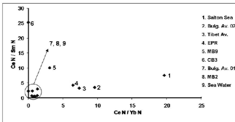
Figure 4 \text{Ce}_\text{N}/\text{Yb}_\text{N} - \text{Ce}_\text{N}/\text{Sm}_\text{N} normalized data. The studied case samples are located into circle with 7, 8, 9 standard data (C1, after [1, 21, 29, 31]).
